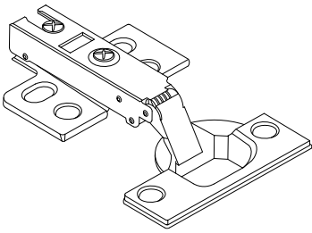
H26 - Scharnier
