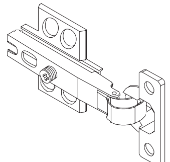
H22 - Scharnier
