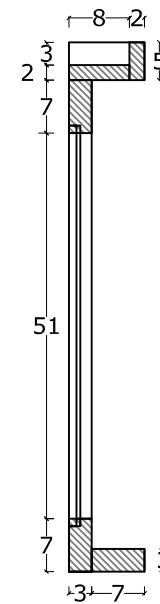
Side Section / Potongan Samping
