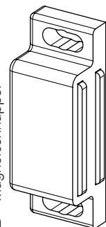
B - Magnetschnapper
