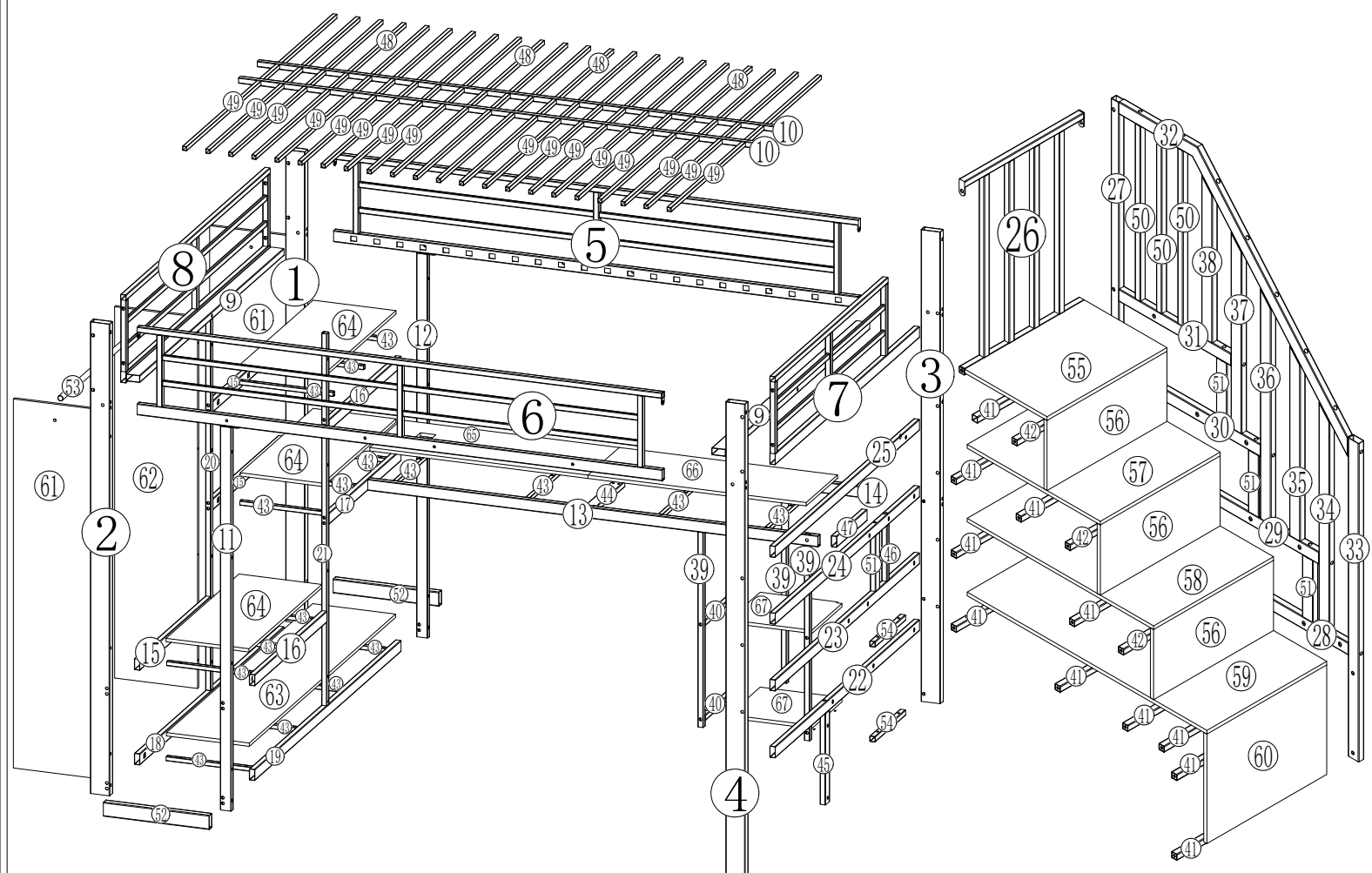
Bed parts view
